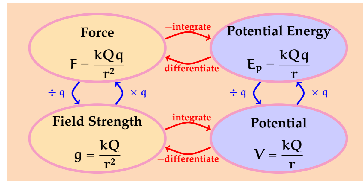
Radial Electric Field
