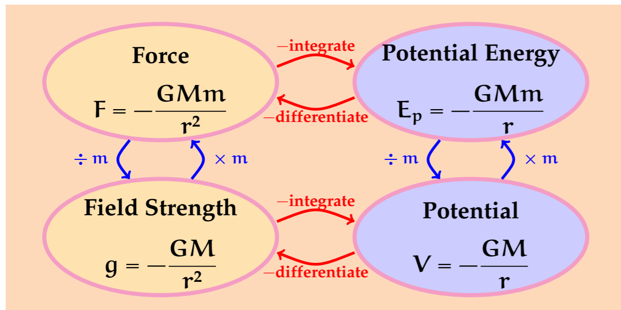
Radial Gravitational Field
